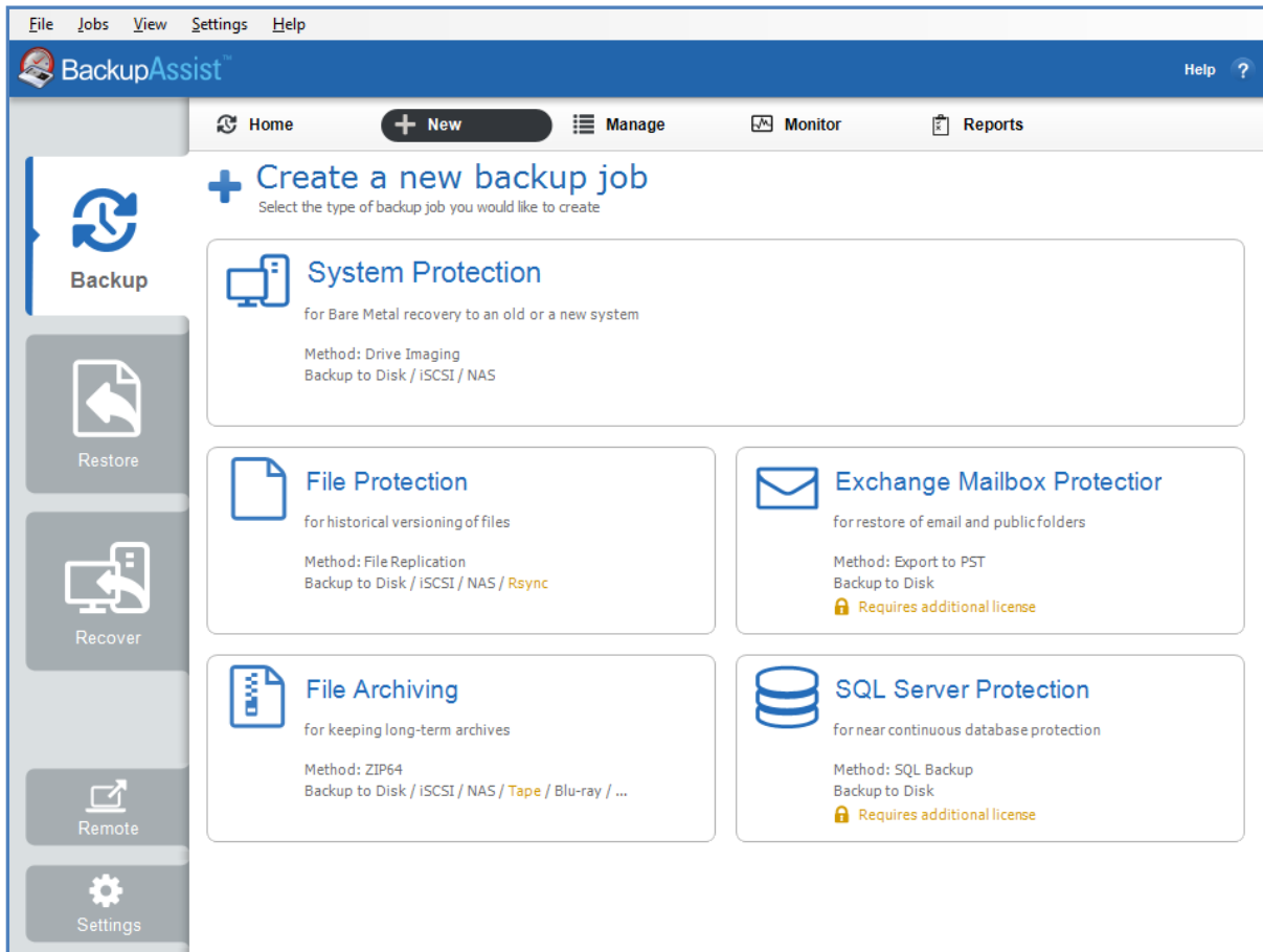
Figure 3: BackupAssist GUI – Backup tab
